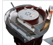
Combo HR Series: Internal separating bowl for heavier duty processes, includes a higher degree of automation.
