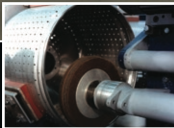
Flap Wheel of Washer Tub
