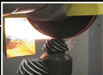
Secondary head in same machine working top of gear.
